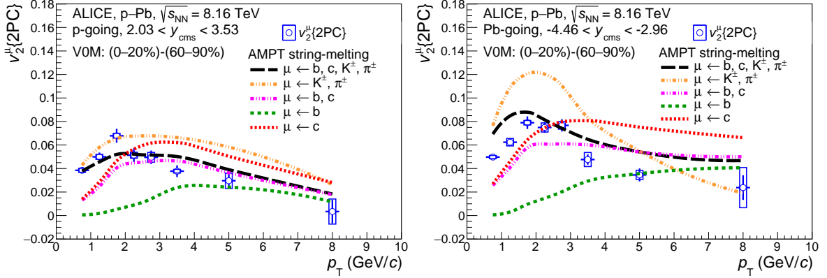
Figure 6: Comparison of the p_T -differential v_2^\mu \{2PC\} of inclusive muons at forward (left) and backward (right) rapidities in high-multiplicity p–Pb collisions at \sqrt{s_{NN}} = 8.16 TeV with AMPT calculations [81–83]. The predictions are shown for muons from charm-hadron decays and beauty-hadron decays, separately, muons from charged-pion and kaon decays, and for muons from the combination of the various sources. The contribution of muons from both charm- and beauty-hadron decays is also displayed.
