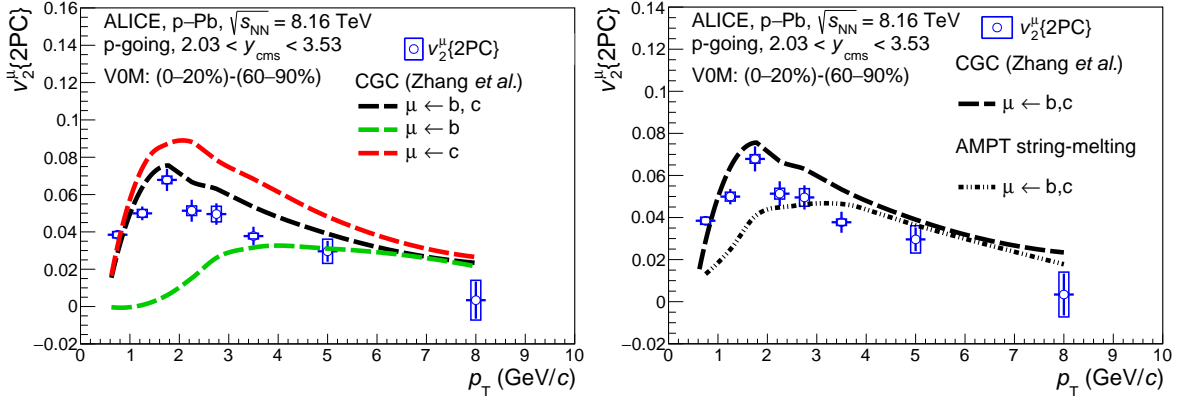
Figure 7: Left: comparison of the p_T -differential v_2^{\mu\{2PC\}} of inclusive muons at forward rapidity in high-multiplicity p–Pb collisions at \sqrt{s_{\text{NN}}} = 8.16 TeV with CGC-based calculations [112, 113]. The predictions are shown for muons from charm-hadron decays and beauty-hadron decays, separately, and for muons from the combination of the two sources. Right: comparison of the p_T -differential v_2 of muons from heavy-flavour hadron decays as obtained with CGC and AMPT calculations with the measured inclusive muon v_2 .
