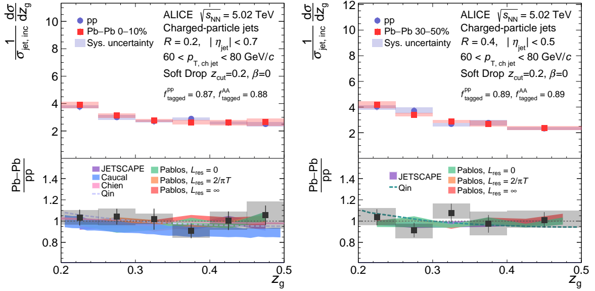
Fig. 2: Unfolded z_g distributions for charged-particle jets in pp collisions compared to those in Pb–Pb collisions at \sqrt{s_{\text{NN}}} = 5.02 TeV with z_{\text{cut}} = 0.2 for 0–10% centrality for R = 0.2 (left) and 30–50% centrality for R = 0.4 (right). The distributions are normalized to the inclusive jet cross section in the 60 < p_{\text{T, ch jet}} < 80 GeV/ c interval, and f_{\text{tagged}} indicates the fraction of splittings that were tagged to pass the SD condition in the selected p_{\text{T, ch jet}} interval. The ratios in the bottom panel are compared to the following theoretical predictions: JETSCAPE [57], Caucal et al. [34, 58], Chien et al. [33], Qiu et al. [35], and Pablos et al. [36, 59, 60].
