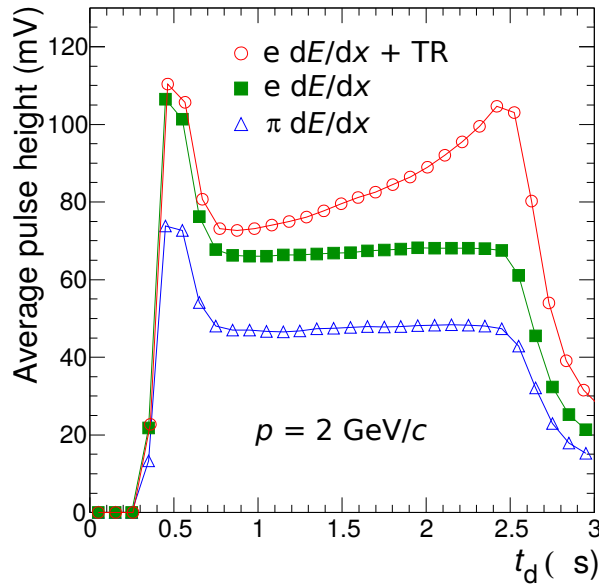
Fig. 5: Average pulse height as a function of drift time for pions and electrons (with and without radiator). The time axis is shown with an arbitrary offset of 0.3 \mu\text{s} . The measurements were performed at the CERN PS with prototype read-out chambers that were smaller in overall size (active area 25 \text{ cm} \times 32 \text{ cm} ) but otherwise similar in construction to that of the final detector. Figure taken from [47].
