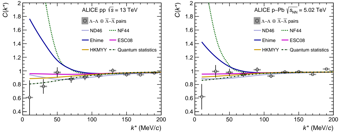
Fig. 2: \Lambda - \Lambda correlations measured in pp collisions at \sqrt{s} = 13 TeV (left panel) and p-Pb collisions at \sqrt{s_{\text{NN}}} = 5.02 TeV (right panel) together with the functions computed by the different models [20]. The tested potentials are converted to correlation functions using CATS and the baseline is refitted for each model. The effects of momentum resolution and residuals are included in the theory curves.
