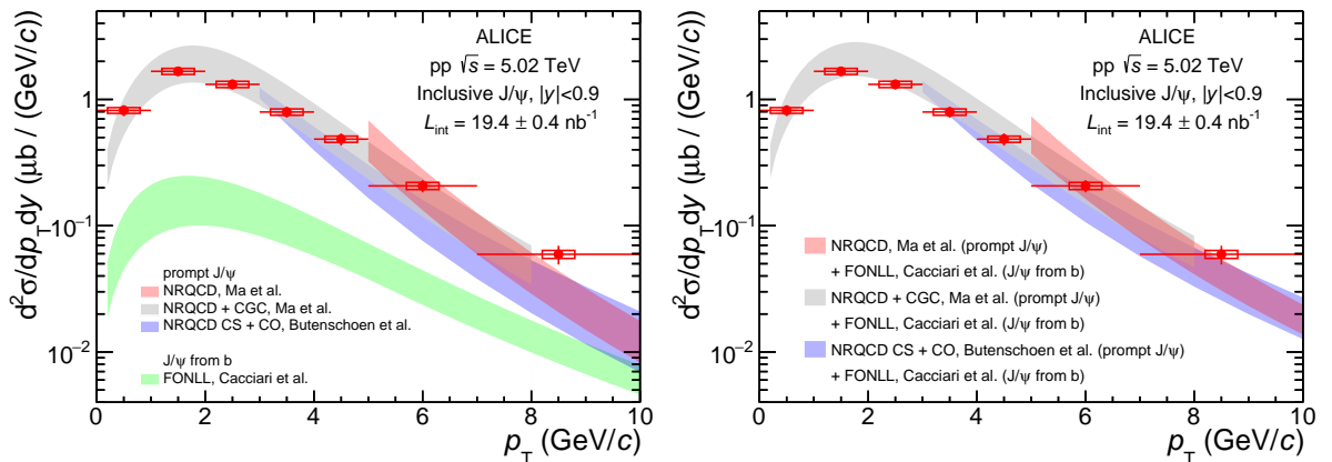
Fig. 3: p_T -differential inclusive J/\psi cross section compared with prompt J/\psi calculations from NLO NRQCD [51, 52] and LO NRQCD+CGC [47] and non-prompt J/\psi calculations from FONLL [48]. The calculations for the prompt and non-prompt components are shown separately in the left panel while in the right panel the FONLL calculation is added to the prompt J/\psi calculations.
