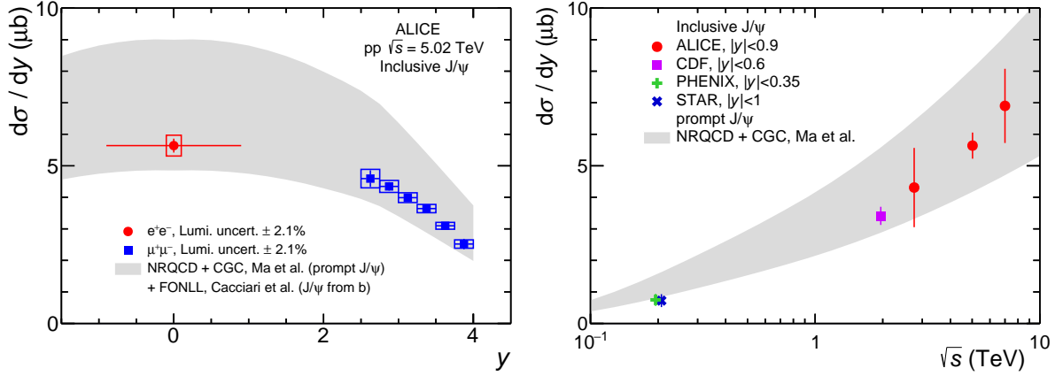
Fig. 2: Left: Inclusive J/\psi cross-section as a function of rapidity compared to the ALICE results at forward rapidity [19] and to calculations from [47] to which a non-prompt component is added as computed in [48]. Right: Inclusive J/\psi cross section at mid-rapidity [15, 16, 38, 49, 50] as a function of collision energy compared to the calculations from [47]. The data points from PHENIX and STAR, both at \sqrt{s} = 0.2 TeV, are slightly shifted for visibility.
