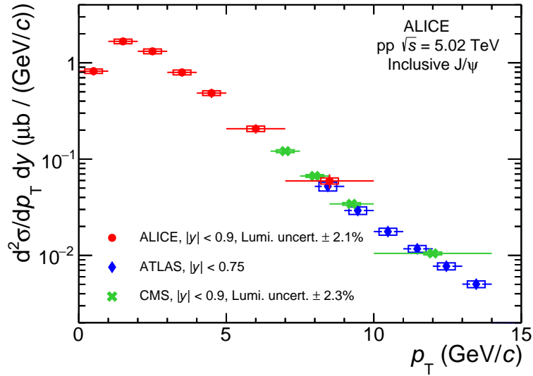
Fig. 4: p_T -differential inclusive J/\psi cross section compared with ATLAS [13] and CMS [14] results at mid-rapidity. Luminosity uncertainties are indicated in the legend, except in the case of ATLAS for which these are included in the boxes.
