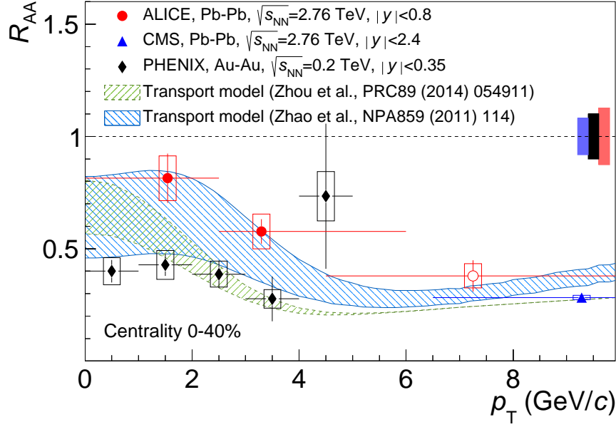
Fig. 6: The nuclear modification factor R_{AA} of inclusive J/\psi , measured at mid-rapidity ( |y| < 0.8 ) in Pb-Pb collisions (0–40% most central) at \sqrt{s_{NN}} = 2.76 TeV, as a function of transverse momentum p_T . The filled symbols are placed at the measured p_T for the given interval. Since for the data point in 4.5 < p_T < 10 GeV/c (open symbol, 0–50% most central) \langle p_T \rangle is not available due to the limited statistics, it is plotted at the centre of the p_T interval. The uncorrelated systematic uncertainties (type II) are depicted by the open boxes, while the correlated uncertainties (type I) are shown as the filled boxes at unity. The data are compared to corresponding results by PHENIX for Au-Au collisions (0–40% most central) at \sqrt{s_{NN}} = 0.2 TeV [9], by CMS for Pb-Pb collisions (0–40% most central) at \sqrt{s_{NN}} = 2.76 TeV [13], and to predictions by the model of Zhou et al. [73] and Zhao et al [74, 75].
