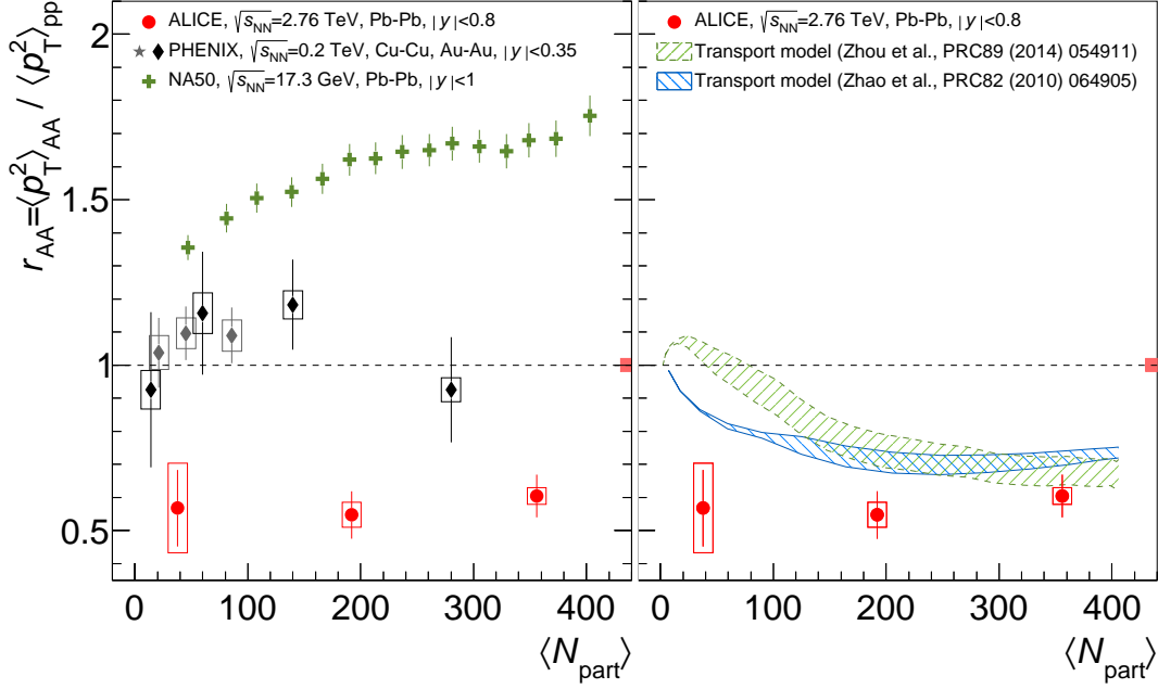
Fig. 5: The ratio r_{AA} = \langle p_T^2 \rangle_{AA} / \langle p_T^2 \rangle_{pp} in the p_T interval 0 – 10 GeV/c for inclusive J/\psi measured at mid-rapidity ( |y| < 0.8 ) in centrality selected Pb-Pb collisions (filled circles) at \sqrt{s_{NN}} = 2.76 TeV as a function of the number of participants \langle N_{part} \rangle . The uncorrelated systematic uncertainties (type II) are depicted by the open boxes, while correlated uncertainty (type I) is shown as the filled box at unity. Left panel: A comparison to results obtained by the PHENIX collaboration for Au-Au and Cu-Cu collisions at \sqrt{s_{NN}} = 0.2 TeV [9, 71] (filled diamonds) and by the NA50 collaboration for Pb-Pb collisions at \sqrt{s_{NN}} = 17.3 GeV [72] (crosses). The PHENIX and NA50 r_{AA} values are calculated in the p_T interval 0 – 5 GeV/c. Right panel: r_{AA} is compared to theory predictions by Zhou et al. [73] and Zhao et al. [74, 75] for the p_T interval 0 – 10 GeV/c.
