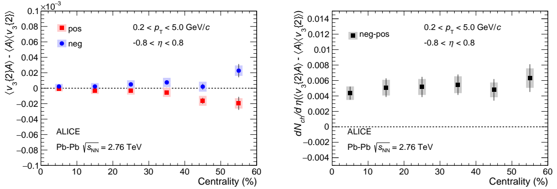
Fig. 5: (Color online) Three-particle correlator for the third harmonic (left panel) for positive (red squares) and negative (blue circles) particles, and the charge difference multiplied by \langle dN_{\text{ch}}/d\eta \rangle (right panel). Statistical (systematic) uncertainties are indicated by vertical bars (shaded boxes).
