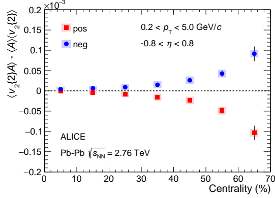
Fig. 3: (Color online) Three-particle correlator for positive (red squares) and negative (blue circles) particles for the second harmonic as a function of centrality. Statistical (systematic) uncertainties are indicated by vertical bars (shaded boxes).
