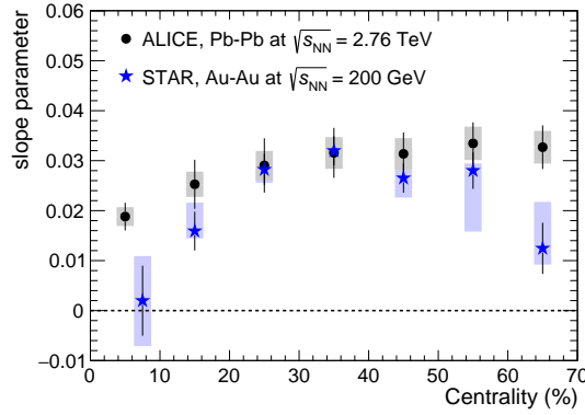
Fig. 7: (Color online) Slope parameter r as a function of centrality, including points from STAR [30]. Statistical (systematic) uncertainties are indicated by vertical bars (shaded boxes).
