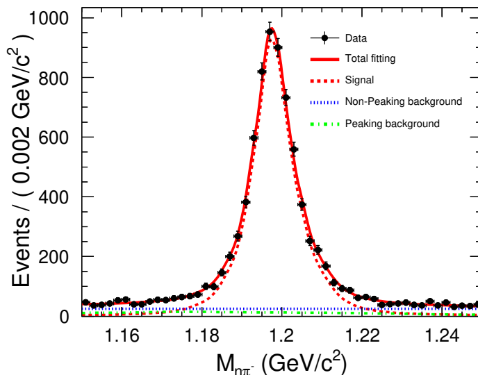
Figure 1. The distribution of M_{n\pi^-} for the process \psi(3686) decay to final state n\bar{n}\pi^+\pi^- . The black dots with error bars are the data, the red solid line is the total fit function, the red dashed line is the signal function, the blue dotted line is the non-peaking background function, and the green dash-dotted line is the peaking background function.
