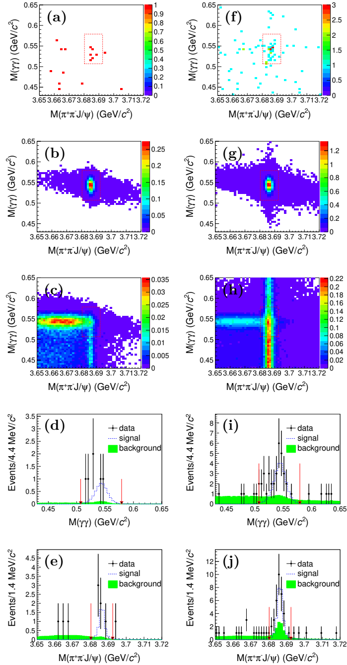
Figure 1. Two-dimensional distributions of M(\gamma\gamma) versus M(\pi^+\pi^-J/\psi) for (a) data, (b) signal MC simulation, and (c) background MC contributions with the red dashed boxes for the defined \eta and \psi(2S) signal regions, and the corresponding projections of (d) M(\gamma\gamma) distribution in the \psi(2S) mass window and (e) M(\pi^+\pi^-J/\psi) distribution in the \eta mass window with red arrows for the defined signal regions at \sqrt{s} = 4.258 GeV, where the dots with error bars, the dashed blue lines, and the green histograms represent data, signal MC, and background MC simulations, respectively. The same distributions for the sum of the 14 data samples and MC samples are shown in (f), (g), (h), (i), and (j) correspondingly.
