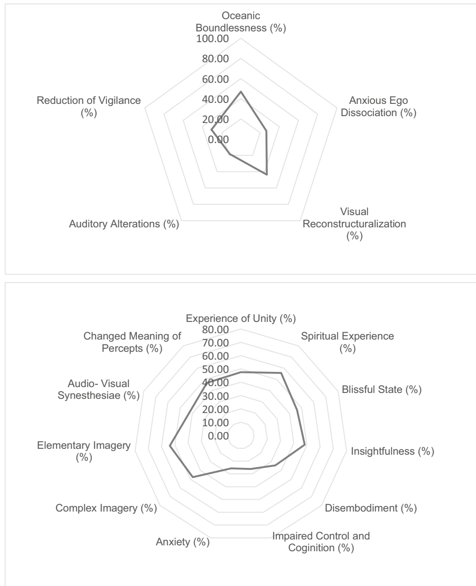
Fig. 4 Mean ratings of the experience of altered states of consciousness as assessed with 5D-ASC (from 0 to 100%) dimensions (top) and subscales (bottom)
