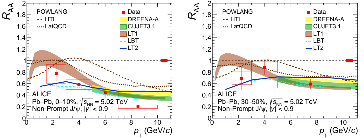
Figure 11: Non-prompt J/\psi R_{AA} as a function of p_T in the 0–10% (left panel) and 30–50% (right panel) centrality classes compared with models [92, 95, 96, 101–104]. Error bars and boxes represent statistical and uncorrelated systematic uncertainties, respectively. Shaded bands represent model uncertainties where applicable. The global uncertainty is shown around unity.
