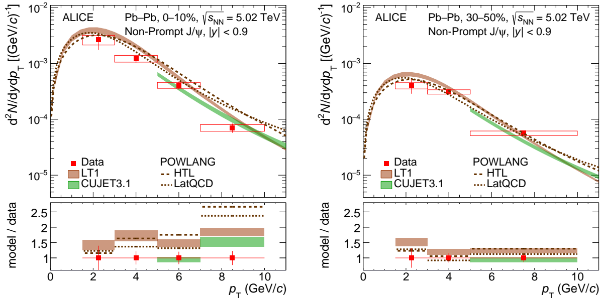
Figure 10: Non-prompt J/\psi yields as a function of p_T in the 0–10% (left panel) and 30–50% (right panel) centrality classes compared with models [92–96]. Vertical error bars and boxes represent statistical and systematic uncertainties, respectively. Shaded bands in the top panels represent model uncertainties where applicable. Bottom panels show the ratios between models and data, with the bands representing the relative uncertainties from the models. Error bars around unity are the quadratic sum of statistical and systematic uncertainties on the measured yields.
