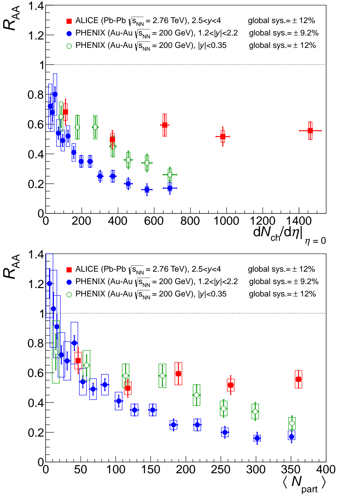
Fig. 2: (Color online) Inclusive J/\psi R_{AA} as a function of the mid-rapidity charged-particle density (top) and the number of participating nucleons (bottom) measured in Pb-Pb collisions at \sqrt{s_{NN}} = 2.76 TeV compared to PHENIX results in Au-Au collisions at \sqrt{s_{NN}} = 200 GeV at mid-rapidity and forward rapidity [4, 5, 20]. The ALICE data points are placed at the dN_{ch}^w/d\eta|_{\eta=0} and \langle N_{part}^w \rangle values defined in Table 1.
