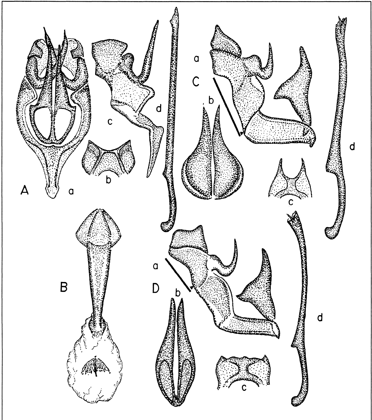
Figure 5. Male genitalia of other Tergissima and Femniterga species and male and female genitalia of sympatric Thecla autoclea . A-B. T. autoclea (Pinchanal, Salta Province, Argentina, AMNH). A) Male genitalia: a. genitalia, ventral view, aedeagus removed; b. uncus, dorsal view; c. genitalia, lateral view, aedeagus removed; d. aedeagus, lateral view. B) Female genitalia: genital plate and corpus bursae, ventral view. C-D. Male genitalia, Tergissima macphersoni , holotype, and Femniterga judae , paratype, respectively. Format: same as Figure 3.
