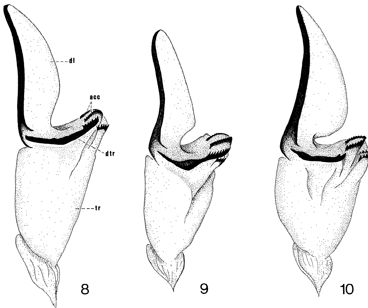
Figures 8-10. Hemispermatothore morphology (dorsal aspect) of Megacormus spp. 8, M. grubbsi , new species, holotype male; 9, M. segmentatus Pocock, male from Fortin de las Flores, Veracruz; 10, M. gertschi Diaz, male from Sierra de Zacapaxtla, Puebla. acc = accessory lobes, dl = distal lamina, dtr = rim of dorsal trough, tr = trunk.
