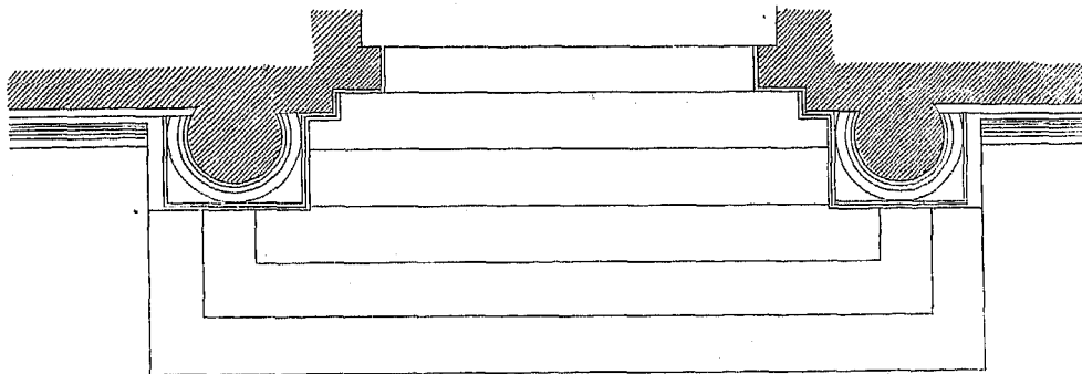
Fig. 287. Thurmportal; Grundriss.
