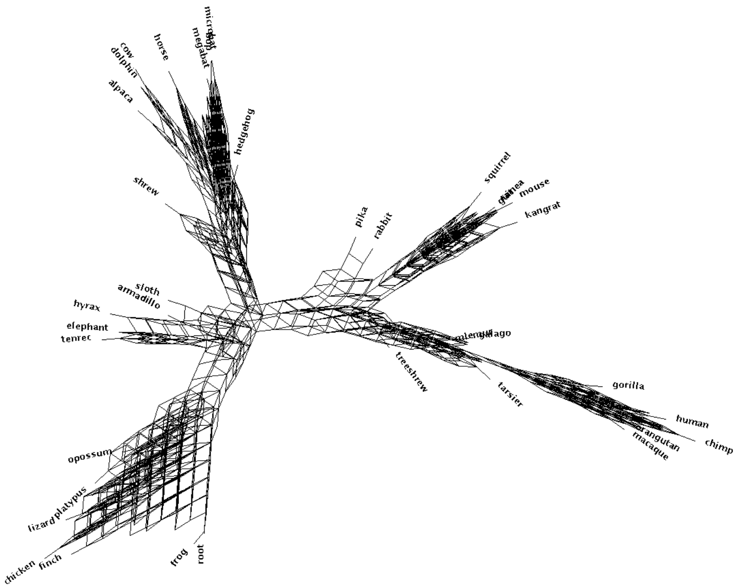
Supplemental figure 2a: Consensus network of 10% longest alignments, threshold = 0.02
