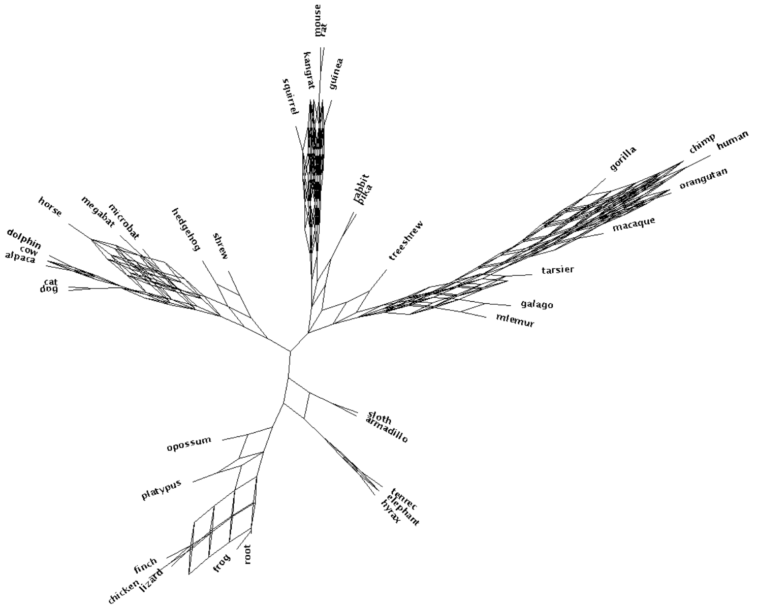
Supplemental figure 2b: Consensus network of 10% longest alignments, threshold = 0.04
