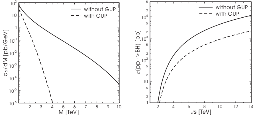
Figure 1. The left plot shows the differential cross section for black hole production in p-p collisions at \sqrt{s} = 14 TeV (LHC) for M_f = 1 TeV. The right plot shows the integrated cross section for BH production as a function of the collision energy \sqrt{s} . In both cases, the curves for various d differ only slightly from the above depicted ones. The dashed curves show calculations including the minimal length (via a Generalized Uncertainty Principle (GUP)) [21, 23].
