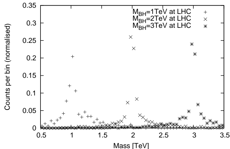
Figure 2. Reconstructed BHR masses in p-p reactions at \sqrt{s} = 14 TeV from ALICE (TOF 56 ps) resolution for M_{\text{BH}} = 1, 2, 3 TeV[27, 49].
