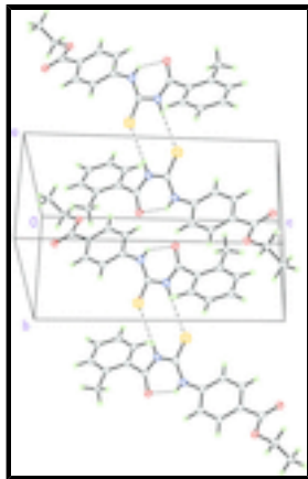
Fig. 2. Packing diagram of the title compound. Hydrogen bonds shown as dashed lines. The minor occupied sites are omitted for clarity.
