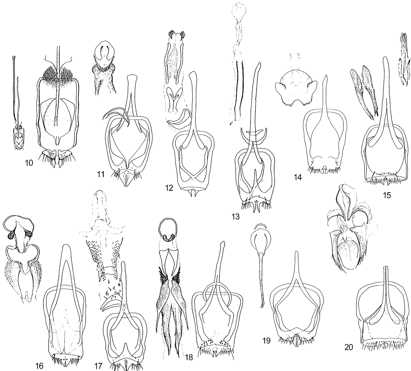
Figures 10-20. Male genitalia, Cryptolestes spp. 10, C. ampyacus , distal (entire aedeagus reduced, inset on left); 11, C. bicolor ; 12, C. capillus ; 13, C. dybasi ; 14, C. mexicanus ; 15, C. pubescens (complete internal sac reduced, inset on right); 16, C. punctatus ; 17, C. schwarzi ; 18, C. spatulifer ; 19, C. trinidadensis ; 20, C. unicornis (all from Thomas 1988)
