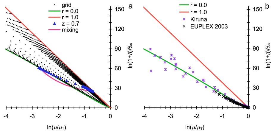
Fig. 13. Same as Fig. 12, but now plotted as \ln(1+\delta) vs. \ln(\mu/\mu_T) .
