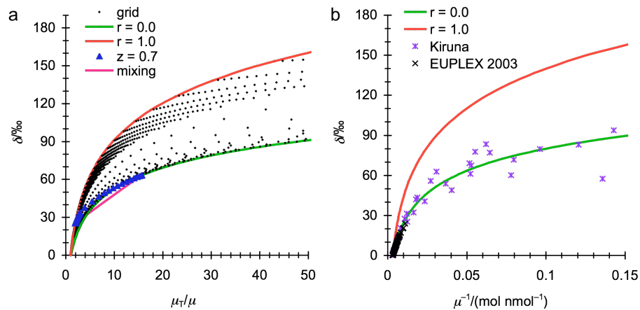
Fig. 14. Same as Fig. 12, but now plotted as \delta value vs. normalized inverse mixing ratio, \mu_T/\mu , or inverse mixing ratio, \mu^{-1} .
