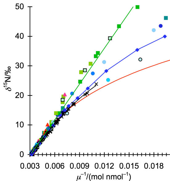
Fig. 10. Linear end-member mixing for some mid-latitude samples, e.g. \delta^{15}\text{N}(\text{ASA } 09/93)=4.0\cdot 10^{-9} \mu^{-1}-12.4\text{‰} ( R^2=0.997 ); weak mixing (?) at polar latitudes, \delta^{15}\text{N}(\text{EUPLEX } 2003)=-1.4\cdot 10^{-16} \mu^{-2}+4.9\cdot 10^{-9} \mu^{-1}-14.2\text{‰} ( R^2=0.998 ). Also shown is a Rayleigh-fractionation curve with a fractionation constant of \varepsilon=-17\text{‰} .
