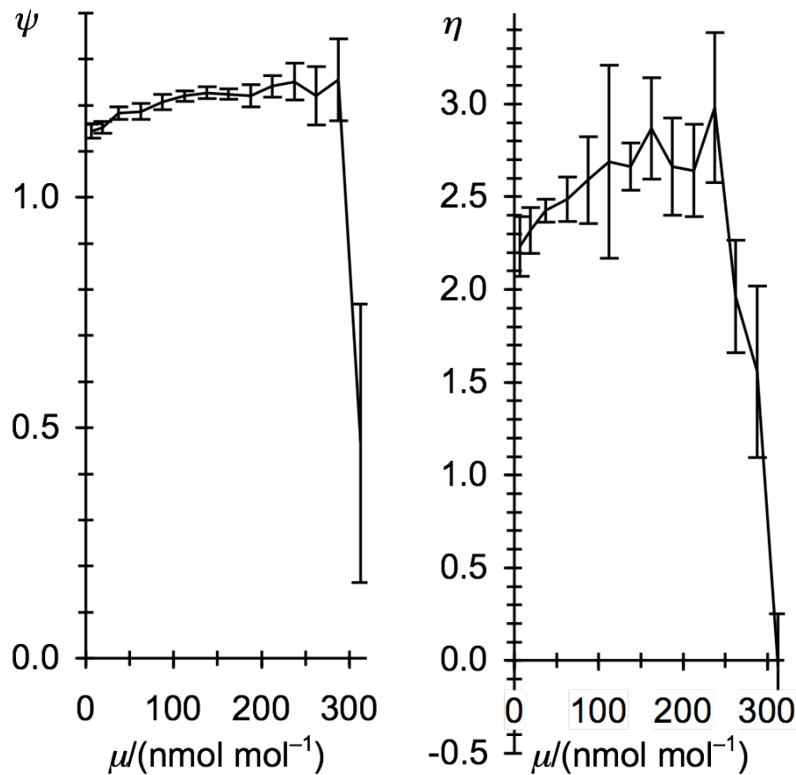
Fig. 15. Dependence of binned \psi - and \eta -values on the N 2 O mixing ratio. Error bars correspond to the standard error of the mean for the respective mixing ratio bin.
