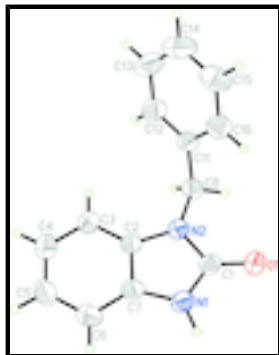
Fig. 1. : Molecular view of the title compound. Displacement ellipsoids are drawn at the 50% probability level. H atoms are represented as small circles of arbitrary radii.
