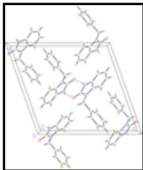
Fig. 2. : Formation of pseudo-dimers between two molecules by N–H...O hydrogen bonds (dashed lines).
