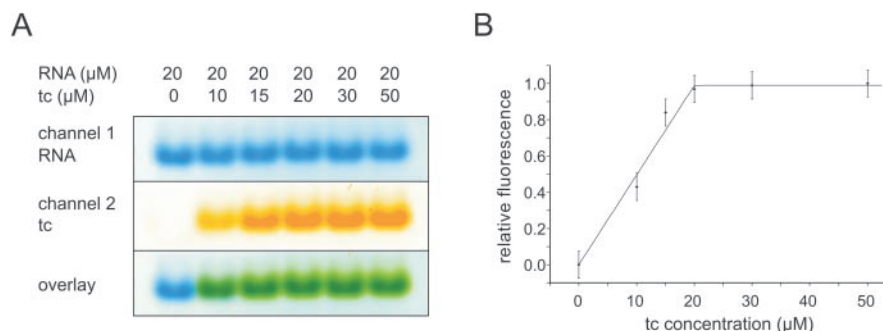
Figure 3. Native PAGE. (A) Visualization of tc-binding (false colors). RNA (20 μM of the minimizer variant) was incubated with increasing amounts of tc and applied to a 10% polyacrylamide gel. Tc was visualized directly by fluorescence (middle panel), RNA subsequently via staining with ethidium bromide (upper panel). Co-localization is demonstrated by the overlay (lower panel). No major conformational changes can be detected between free and complexed RNA. (B) Densitometric quantification. Saturation at 20 μM tc supports an equimolar stoichiometry.
