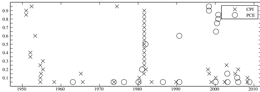
Figure 5: Estimated break points at different quantiles (monthly). Notes: The graph shows breakpoints estimated with the SQ_{\tau} -test at all quantiles \tau \in \{0.05, 0.1, \dots, 0.95\} (vertical axis) for CPI and PCE inflation.
