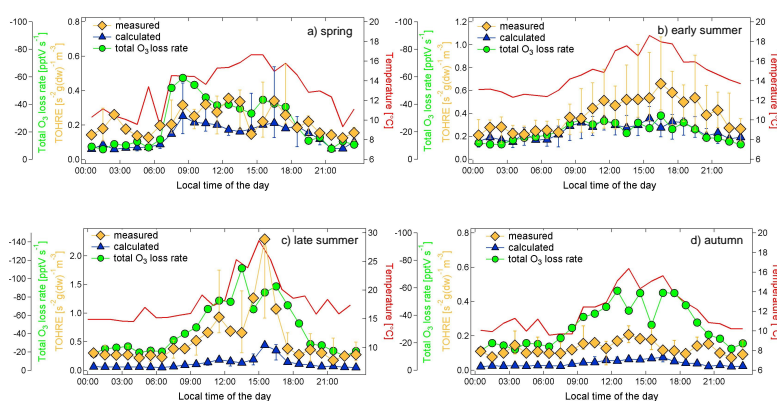
Fig. 6. Median diel profiles for four periods (a) spring, (b) early summer, (c) late summer, (d) autumn of total OH reactivity emissions (TOHRE) which were measured by CRM (orange markers) and calculated from PTR-MS data (blue markers) and of the observed total ozone loss rate (green markers). Additionally, the median temperature profile is included (red line). Uncertainties of the hourly median are given for measured and calculated TOHRE as 75 and 25 percentiles.
