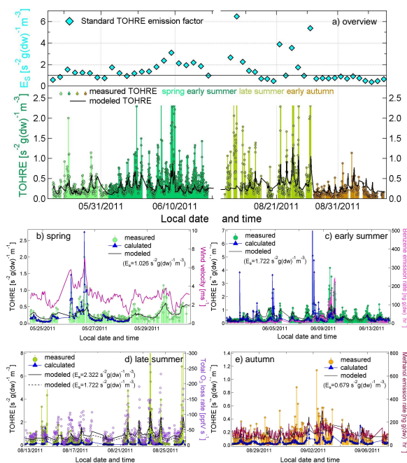
Fig. 8. Overview for model, calculation and measurement comparison of TOHRE: (a) The entire campaign has been modeled (black line) using an unscaled temperature-only dependent algorithm to compare to measured TOHRE (markers on sticks), superimposed the daily standard total OH reactivity emission factor is pictured. Each of the other graphs (b–e) presents measured, calculated and modeled TOHRE as well as one parameter such as wind velocity, benzene emission rates, total O 3 loss rate and methanol emission rates.
