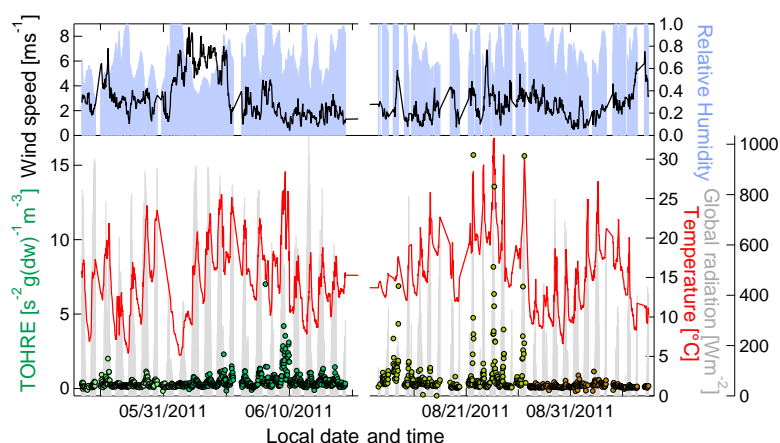
Fig. 3. Overview of the entire data set: Total OH reactivity emissions (TOHRE, green markers) were measured from 24 May to 14 June 2011 and 12 August to 7 September 2011 covering the seasonal impact from spring to early autumn. Temperature inside the cuvette (red line) and global radiation from a co-located mast (grey area) showed high variability throughout the measurement period as well as wind speed (black line, top panel) and relative humidity (blue area, top panel).
