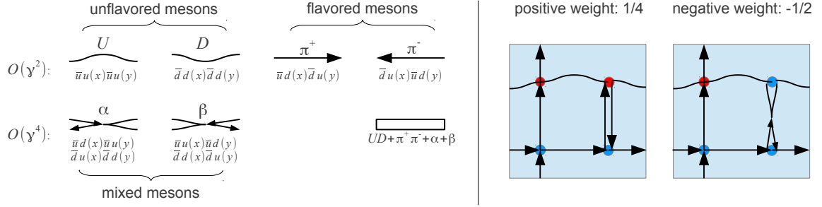
Figure 3: Left: definition of unflavored, flavored, and mixed dimers. Right: 2x2 sample configurations with positive and negative weight.
