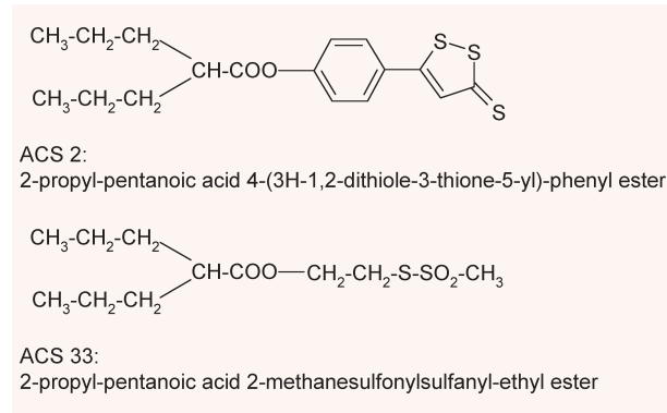
Fig. 1 Chemical structures of histone deacetylase (HDAC)-inhibitors ACS2 and ACS33.
