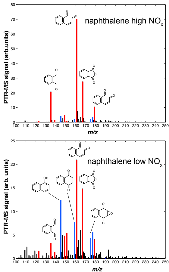
Fig. 3. PTR-MS spectra under high- and low-NO x conditions. The fractions of naphthalene reacted are 0.66 and 0.67, respectively. The red peaks indicate ions associated with ring-opening products, and the blue peaks indicate those associated with ring-retaining products. The proposed structures for these ion peaks are given in Fig. 4.
