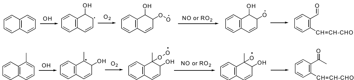
Fig. 6. Mechanism for oxidation of naphthalene and 1-MN to form first-generation dicarbonyl fragmentation product (Wang et al., 2007).
