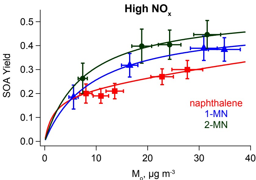
Fig. 7. SOA yield as a function of organic loading for naphthalene, 1-MN and 2-MN under high- \text{NO}_x conditions. The fitting parameters used are summarized in Table 3. Under low- \text{NO}_x conditions, the SOA yields are essentially constant.
