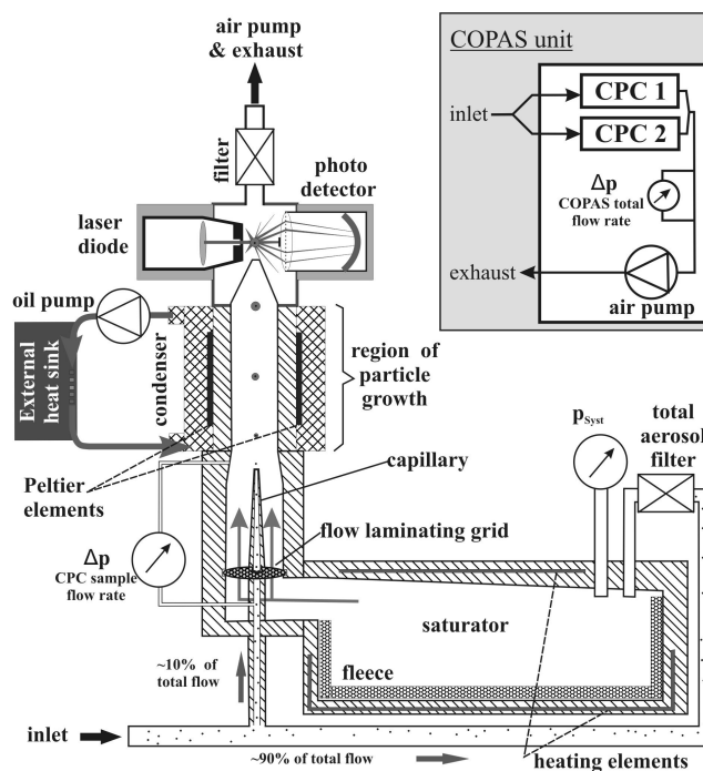
Fig. 1. Flow scheme of a COPAS CPC channel. Two of these counter channels are implemented in one COPAS instrument unit. Two COPAS units (with two CPC channels each) are mounted at different locations on the M-55 “Geophysica”.
