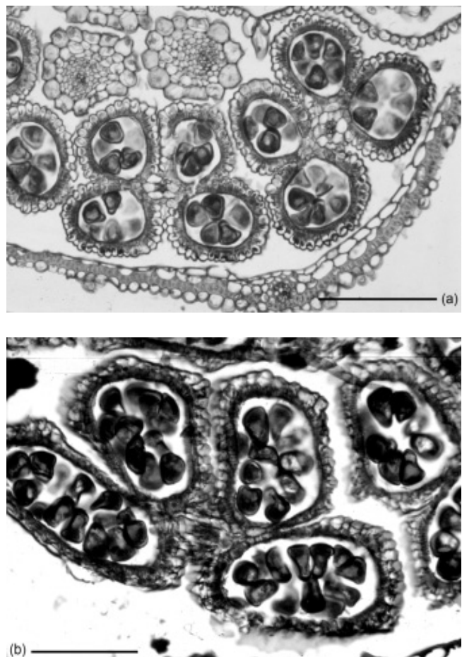
Fig. 1. Transverse sections of mature anthers of (a) Gahnia insignis and (b) Gahnia clarkei . Scale = 25µm.
