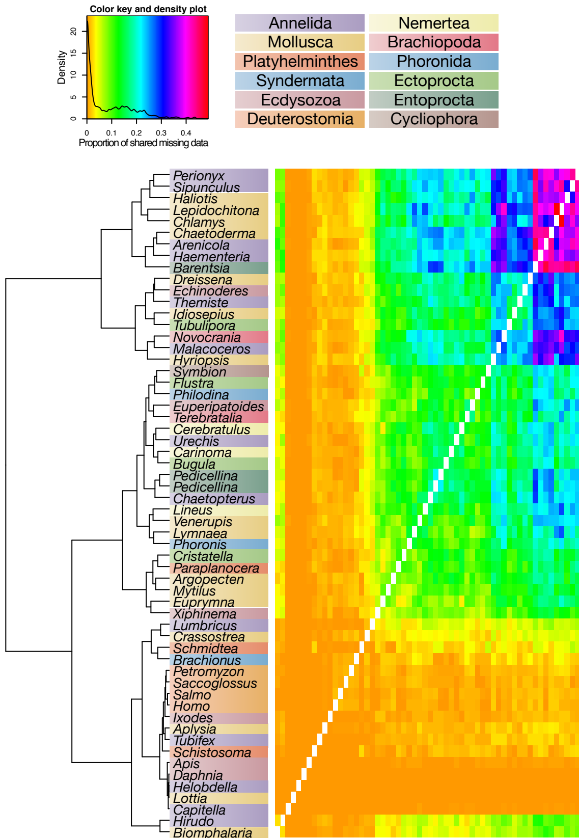
Supplementary Fig. S2. Heat map analysis combined with hierarchical clustering of the reduced dataset of the degree of overlap in missing data shared between taxa. The order of the taxa from left to right along the x-axis is the same as from bottom to top along the y-axis. The higher taxonomic unit of each species is highlighted as indicated in the legend on top. Colours in the heat map indicate proportion of shared missing data ranging from 0 (orange) to 0.5 (red) (see key in upper left corner). The density distribution of the proportions is given in the upper left corner.
