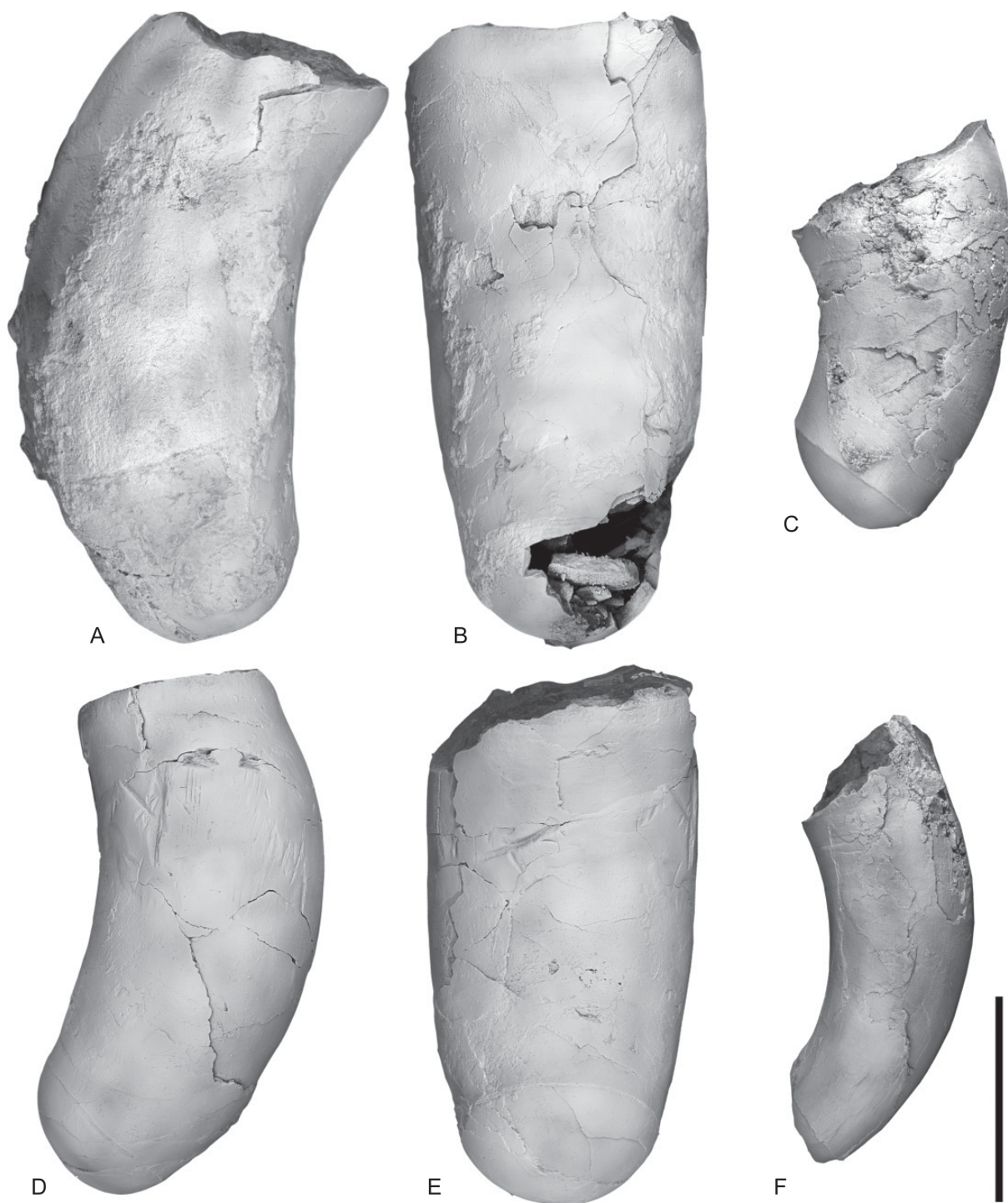
Fig. 43. Redpathoceras Flower, 1963, Kallholn, Boda Limestone. A-C. Redpathoceras magnum sp. nov. A. PMU 26935, holotype; mature truncated body chamber, lateral view. B. Same specimen, view from antispinhuncular side. C. PMU 26946, premature truncated phragmocone, lateral view. D-F. Redpathoceras depressum sp. nov. D. PMU 26927, holotype; mature truncated body chamber, lateral view. E. Same specimen, view from antispinhuncular side. F. PMU 26931, premature truncated phragmocone, lateral view. Scale bar = 50 mm for all figures.
