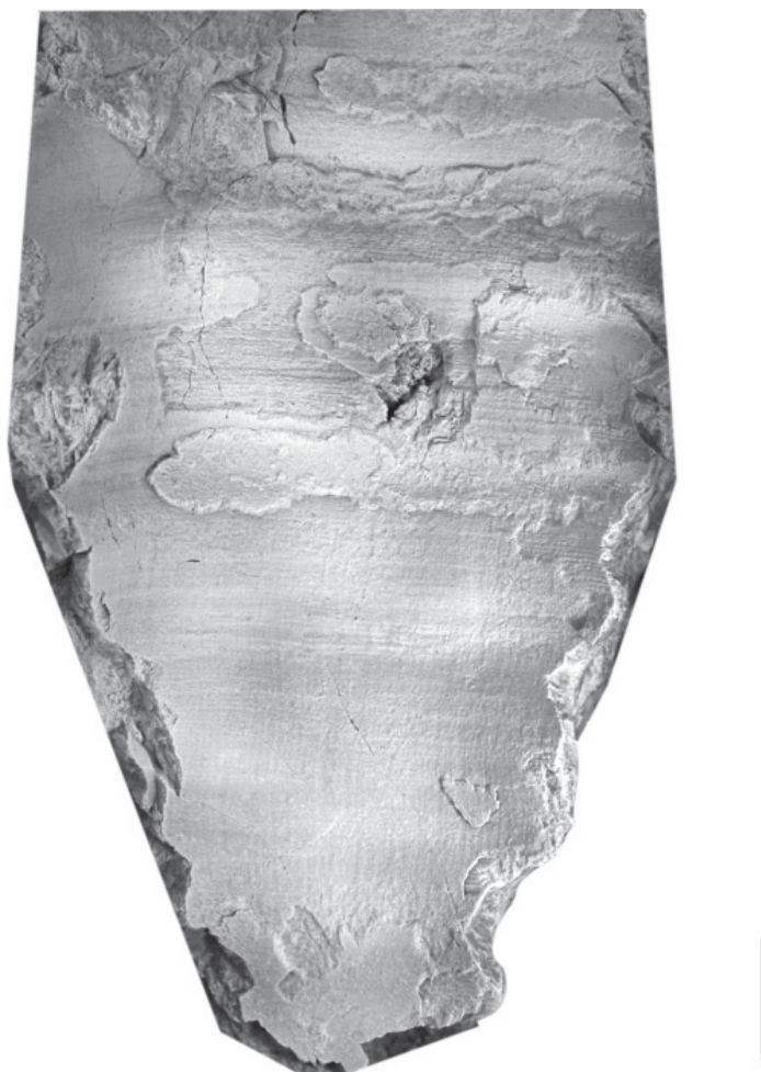
Fig. 15. Fragments of the outer shell and negative shell impression of Striatocycloceras? sp., PMU 26699, Kallholn, Boda Limestone. Scale bar = 10 mm.
