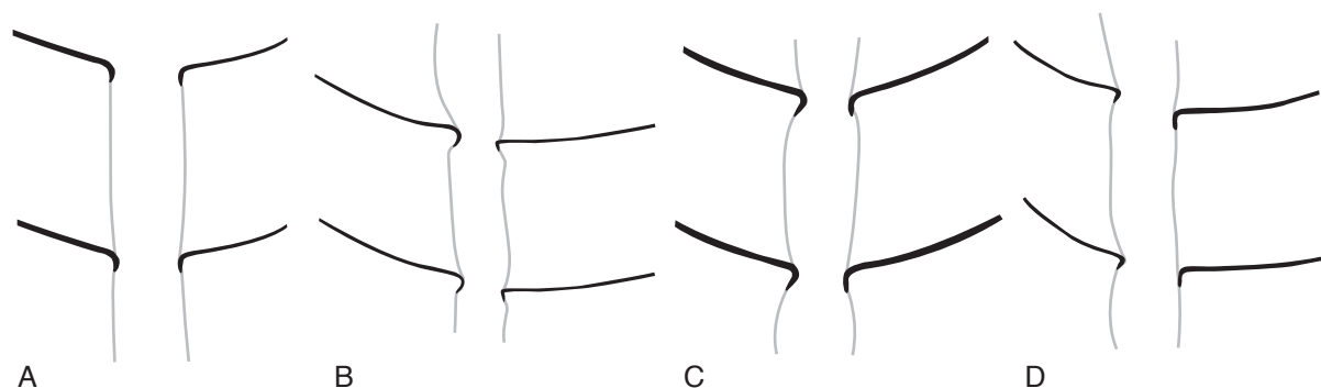
Fig. 14. Reconstructions of the details of the septal necks and siphuncular segments of Orthocerida of the Boda Limestone. Note the different septal thicknesses. A. Striatocycloceras isbergi sp. nov., PMU 26681, Kallholn. B. Dawsonoceras fenestratum (Eichwald, 1860), PMU 26706, Kallholn. C. Pleurorthoceras osmundsbergense sp. nov., NRM-PZ Mo 150102c, Osmundsberget. D. Isorthoceras angelini sp. nov., PMU 26784, Kallholn.
