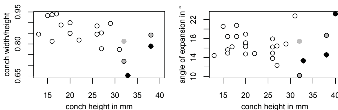
Fig. 11. Morphological variation of Beloitoceras sinuososeptatum (Roemer, 1861). Circles: specimens of the Boda Limestone. Black dot: type specimen of Beloitoceras siljanense Frye, 1987. Black diamonds: types of Beloitoceras heterocurvatum Strand, 1934. Grey dot: type specimen of Beloitoceras landerense Foerste, 1935. A distinction between B. siljanense and B. sinuososeptatum is impossible based on the available material.
