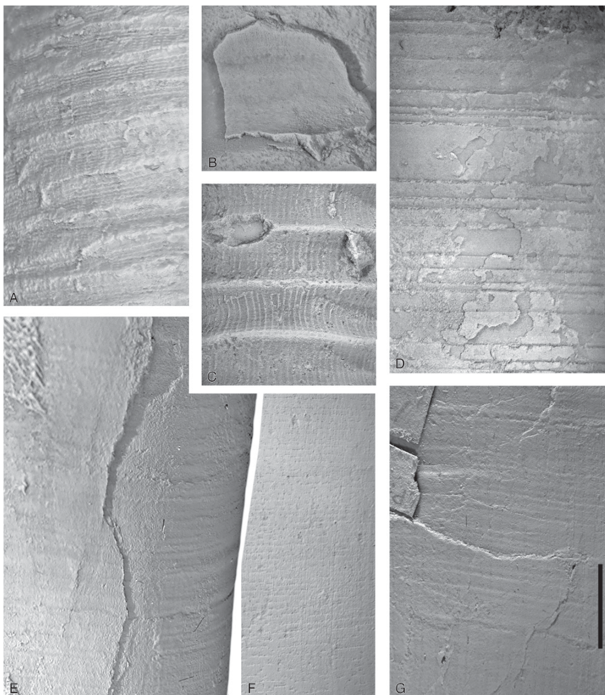
Fig. 18. Shell ornamentation of selected Cephalopoda of the Boda Formation. A. Order, gen. et sp. indet., PMU 26950, Kallholn, lateral view. B. Palaeodawsonocерina? nicolletoides sp. nov., PMU 26727, holotype, Kallholn. C. Palaeodawsonocерina senckenbergi (Teichert, 1930), PMU 26718, Kallholn. D. Geisonoceras wegelini (Angelin in Angelin & Lindström, 1880) comb. nov., PMU 26745, Unskarsheden. E. Pleurorthoceras osmundsbergense sp. nov., NRM-PZ Mo 150126, holotype, Osmundsberget. F. Warburgoceras longitudinale (Angelin in Angelin & Lindström, 1880) comb. nov., NRM-PZ Mo 154065, Unskarsheden. G. Redpathoceras depressum sp. nov., PMU 26931, Kallholn. Scale bar = 5 mm for all figures.
