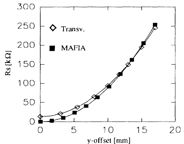
Fig. 5. Longitudinal shuntimpedance measured against y-off-axis position including transittime, MAFIA values weighted with Q_{\text{exp}}/Q_{\text{num}} .
