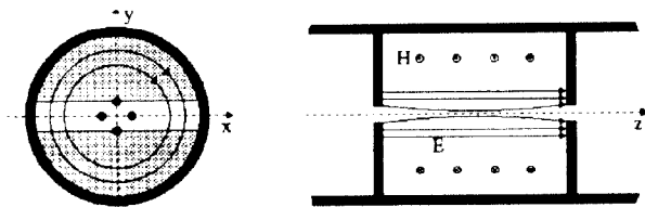
Fig. 1. rf-Quadrupole in TM 010 -π/2-mode
