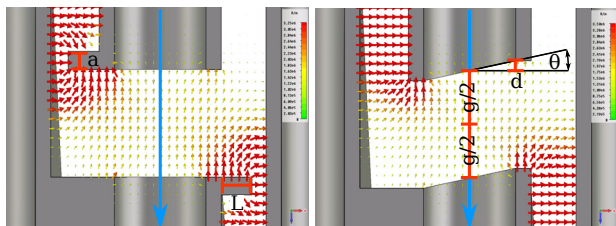
Figure 5: Two different approaches to reducing the deflecting field component within the gaps of the multiaperture rebuncher: bulges and slanted gaps.
