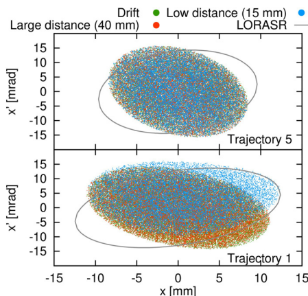
Figure 7: Emittance equivalent homogeneous distribution after transport through the final focus-rebuncher for different distances between trajectory and drift tube side.
