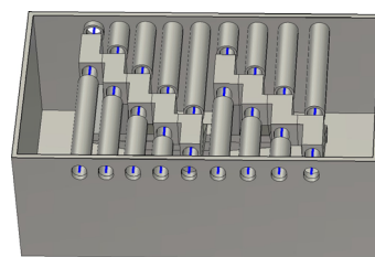
Figure 2: Multiaperture rebuncher cavity design.
