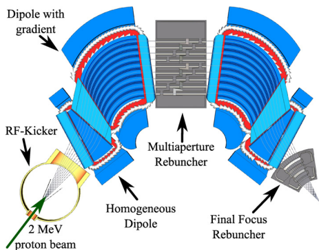
Figure 1: Design of the ARMADILLO. See [2] for details.
