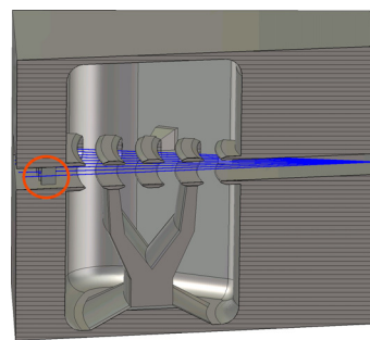
Figure 3: Final Focus cavity with shorting bars.
