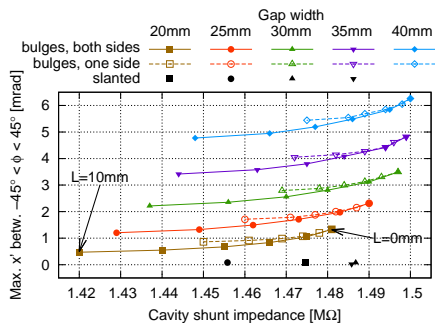
Figure 6: Shunt impedance vs. deflection for cases shown in Fig. 5. Bulge length L varies from 0 mm to 10 mm.
