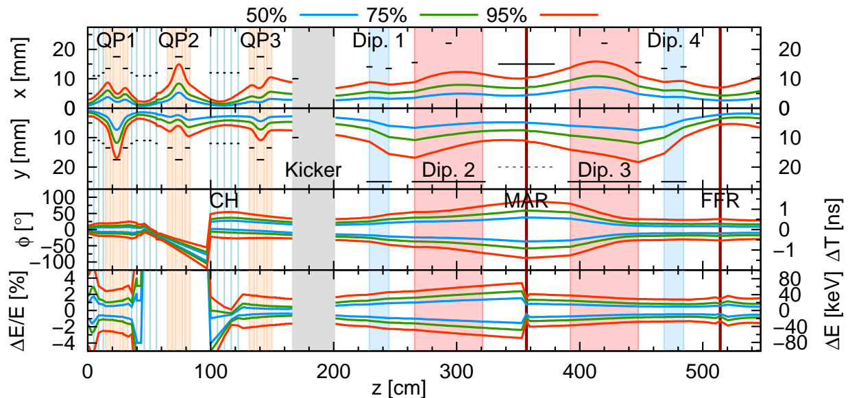
Figure 4: Beam dynamics in the FRANZ linac and the adjoining bunch compressor on the fifth trajectory. Areas where apertures were included in the PSO cost function are marked by horizontal black lines.
