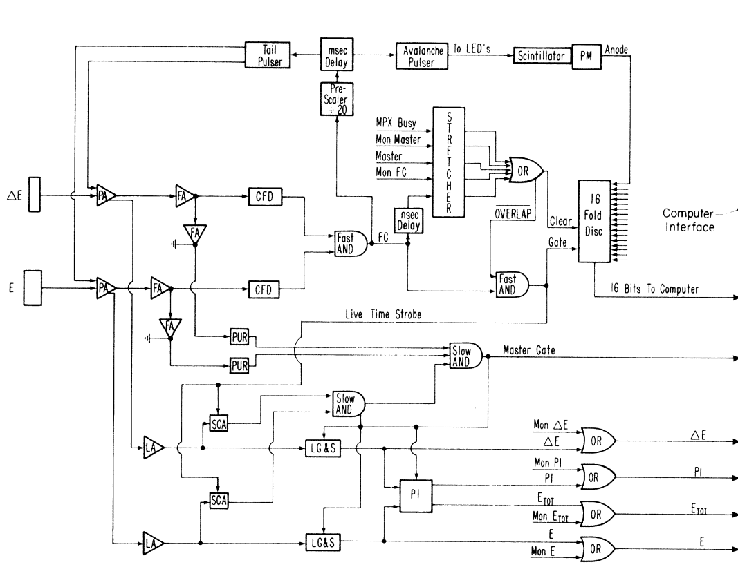
FIG. 4. Simplified electronic diagram representing the fast and slow logic used with both Si-plastic and Si-Ge telescopes. An "alive" signal was used to gate the linear signals as described in the text.
