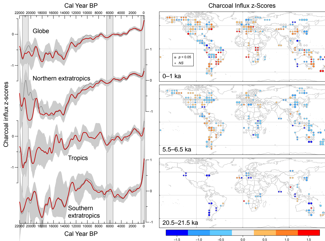
Figure 6. Trends in biomass burning (left panel) from 22 to 0 ka from the GCDv3 (red) and GCDv2 (gray; Daniua et al., 2012) for the entire globe, northern extratropics ( > 30^\circ N latitude), tropics ( > 30^\circ N latitude and < 30^\circ S latitude), and the southern extratropics ( < 30^\circ S latitude), along with spatially gridded charcoal influx z scores reflecting biomass burning (right panel) for the periods 0–1, 5.5–6.5, and 20.5–21.5 ka. Vertical gray bars on the left panel correspond to the intervals shown in the maps (right panel). The charcoal influx anomaly base period for all panels is 21 ka–200 cal yr BP; the smoothing window width is 1000 years. Bootstrap-by-site confidence intervals (95 %) are filled in gray.
