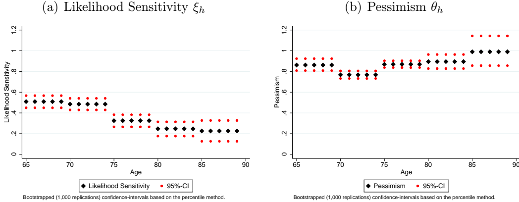
Figure 5: Estimated Prelec Parameters: Likelihood Sensitivity and Pessimism
