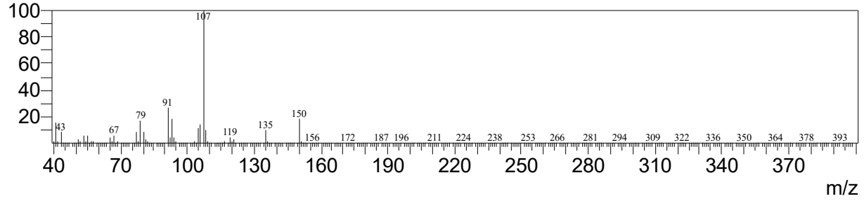
S6 Fig. Mass spectra of all compounds with unknown structure listed in Table 3 or S2 Table
