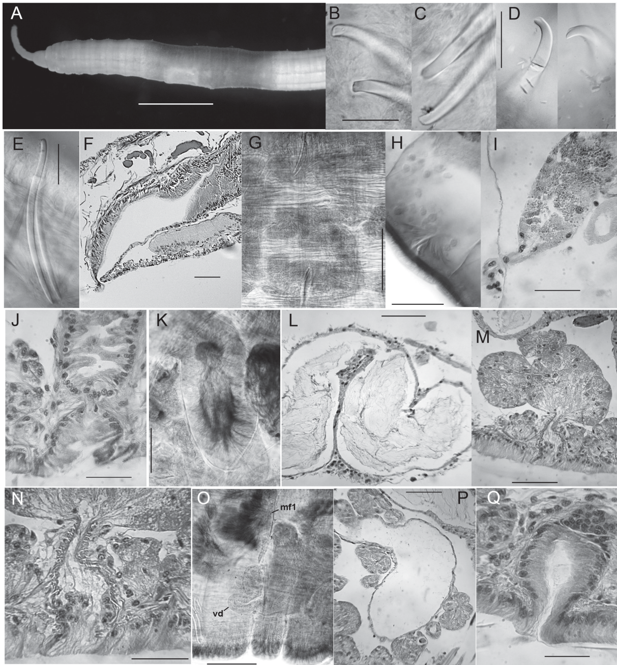
Fig. 9. Guestphalinus exilis Fend & Rodriguez sp. nov., from Squaw Creek (the type locality); F, I–N, P–Q from sagittal sections. A. A complete worm, anterior end, lightly stained with hematoxylin, showing clitellum and genital field. B. Tips of chaetae in II dorsal. C. Chaetae in II ventral. D. Tips of chaetae in two posterior segments, showing dorsal keel. E. Chaetae in II dorsal. F. Pharynx. G. Pharyngeal glands from a whole mount, 3 lobes facing anterior (to left). H. Eleocytes, in a posterior segment. I. Nephridial funnel (left) and postseptal expansion. J. Spermathecal pore and constricted ectal end of duct. K. Spermathecal ampulla, ectal part, with sperm penetrating epithelium. L. Spermathecal ampulla, ental part with weakly-staining sperm. M. Ventral copulatory gland. N. Pore of copulatory gland. O. Anterior vas deferens protruding into VII (to left), with male funnel on 8/9. P. Expanded atrial ampulla with prostates. Q. Male pore. Scale bars: A = 2 mm; B–E, H–J, N, Q = 50 µm; F–G, K–M, O–P = 100 µm.
