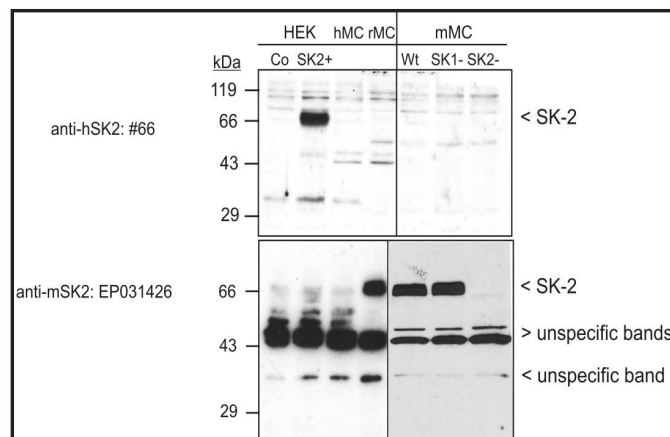
Fig. 1. Characterization of the species specificities of mSK-2 and hSK-2 antibodies in mesangial cells. Untransfected HEK293 cells (Co), or HEK293 cells overexpressing hSK-2 (SK2+), human (hMC), rat (rMC), and mouse mesangial (mMC) cells isolated from C57BL/6 mice (Wt), SK-1 deficient mice (SK1-) and SK-2 deficient mice (SK2-) were taken for protein extraction and separation, and subjected to Western blot analysis using antibodies against mSK-2 (EP031426; dilution 1:1000) (lower panel) or hSK-2 (#66; dilution 1:1000, upper panel). Bands were visualized by the ECL method according to the manufacturer’s instruction.
