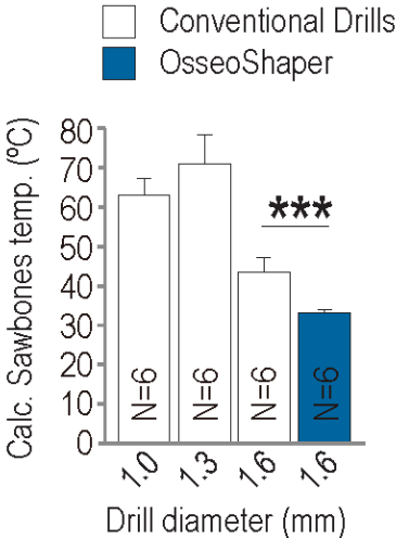
Figure S1. Thermal radiation measurements of conventional and Osseoshaper protocols in Sawbones. In the conventional protocol, the heat radiating from conventional drills was significantly higher for each step compared to the heat radiating from the mini OsseoShaper. Three asterisks indicate p < 0.001 .
