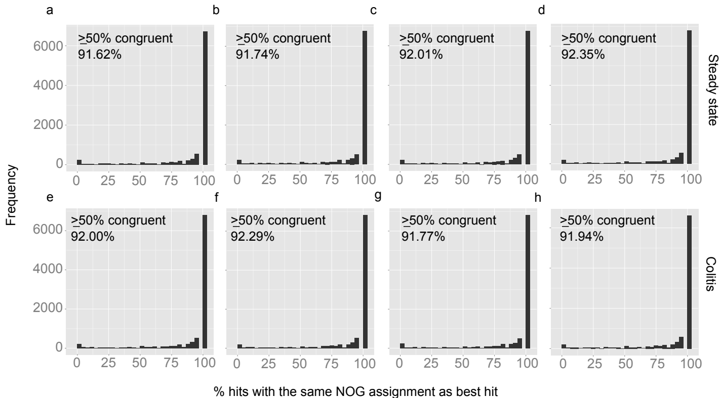
Supplementary Figure S1. DIAMOND best hit NOG is representative of additional hits. Histograms representing the distribution of percent congruency of alignment hits to the best hit for a sample of 10,000 aligned reads. In all cases, the majority of additional hits ( \geq 50\% ) are congruent with the best hit in terms of NOG assignment.
