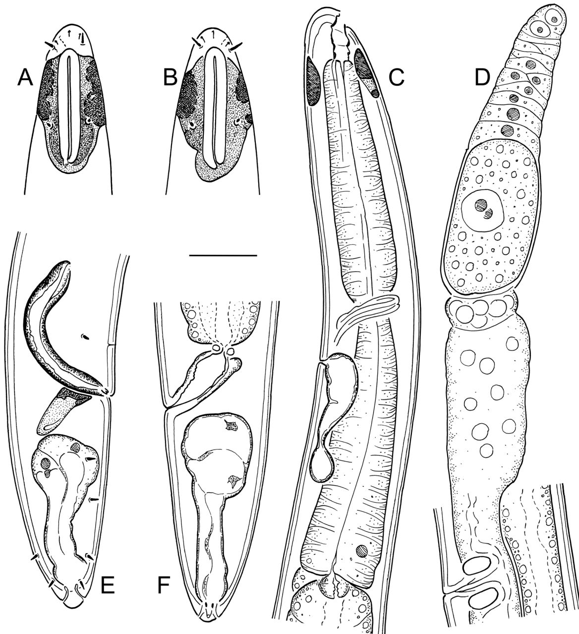
Fig. 8. Neodiplopettula onusta (Wieser, 1956) gen. et comb. nov. (SMNH-169282). A. Male anterior end, surface view. B. Female anterior end, surface view. C. Female pharyngeal region, optical median section. D. Anterior part of female reproductive system. E. Male tail. F. Female tail. Scale bar = 20 \mu\text{m} .
