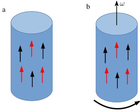
Fig. 1. (Color online) a) a macroscopic fluid at rest with polarized particles (black arrows) and antiparticles (red arrows). This situation, even if metastable, requires a spin tensor to be described, b) if the spin tensor vanishes, the fluid must be rotating (non-vanishing thermal vorticity) to have polarized particles and antiparticles in the same direction.
