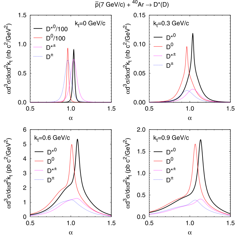
Fig. 6. The invariant differential cross sections of D^{*0} , D^0 , D^{*\pm} and D^{\pm} production in \bar{p}^{40}\text{Ar} collisions at p_{\text{lab}} = 7 GeV/c. The calculations are done using full cross section X(3872)p \rightarrow D^*(D) in Eq. (28) including the IA term as well as screening and antiscreening corrections (see Eqs. (17)–(19)). For k_t = 0 , the cross sections of D^{*0} and D^0 production are divided by a factor of 100.
