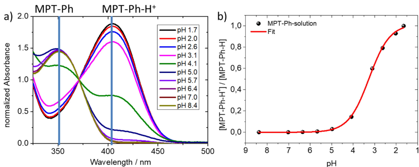
Figure 5. (a) UV-vis spectra of MPT-Ph at pH values between 8.4 and 1.7; (b) corresponding plot to measurements from (a), showing the quotient of MPT-Ph- H^+ / MPT-Ph plotted against the solution pH value (black spheres). The red line shows a mathematical sigmoidal fit to determine the pKa value of MPT-Ph (pKa=3.3).
