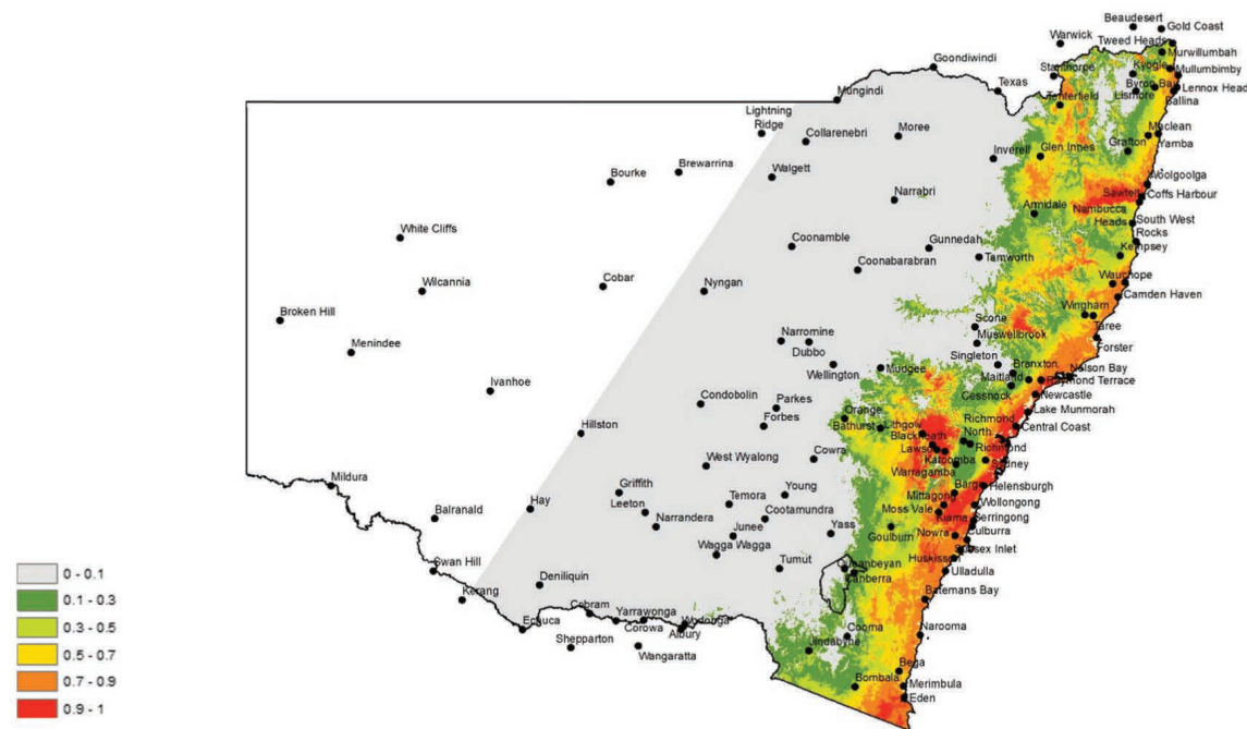
Fig. 8. Habitat suitability for Phytophthora cinnamomi under representative concentration pathway 4.5 (averaged over three climate models and ranked from 0 = unsuitable to 1 most suitable). The unshaded area was not assessed in the model as there were no presence or absence data there.
