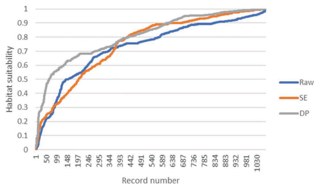
Fig. A2. Habitat suitability of presence records for Phytophthora cinnamomi in NSW with no data cleaning (Raw) and cleaning approaches based on sampling intensity (SE) and area (DP). Very few presence records using the DP cleaning approach were assigned very low habitat suitability (< 0.3); i.e. omission was low compared to the other approaches.
