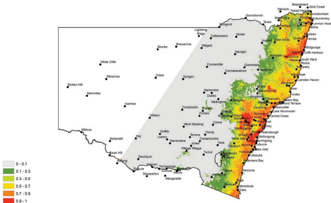
Fig. 7. Current habitat suitability for Phytophthora cinnamomi (ranked from 0 = unsuitable to 1 most suitable). The unshaded area was not assessed in the model as there were no presence or absence data there.
