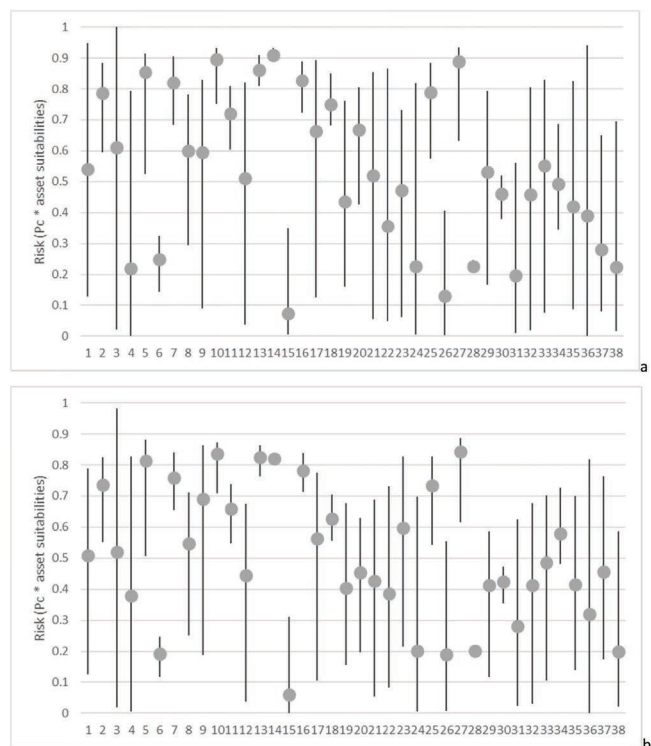
Fig. 15. Minimum to maximum risk for Protected Areas with 10 or more samples for Phytophthora cinnamomi (line) and mean risk (grey dot), a) currently and b) in 2070 under representative concentration pathway 4.5: 1. Barrington Tops NP, 2. Berowra Valley NP, 3. Blue Mountains NP, 4. Border Ranges NP, 5. Brisbane Water NP, 6. Bungonia NP , 7. Dharawal NP , 8. Dharug NP , 9. Dorrigo NP, 10. Garigal NP , 11. Georges River NP ,
