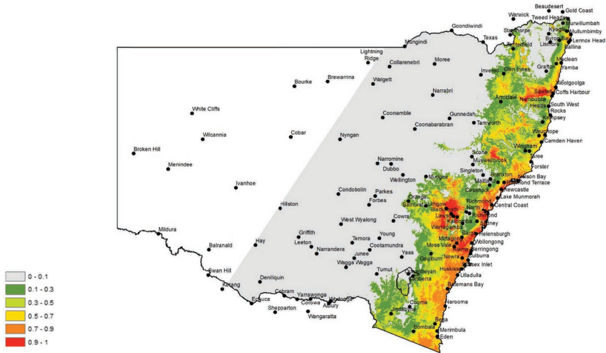
Fig. 9. Habitat suitability for Phytophthora cinnamomi under representative concentration pathway 8.5 (averaged over three climate models and ranked from 0 = unsuitable to 1 most suitable). The unshaded area was not assessed in the model as there were no presence or absence data there.
