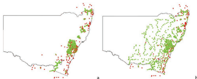
Fig. 2. Location of records of Phytophthora cinnamomi in NSW, northern Victoria and southern Queensland used for modelling in this paper, a) recorded prior to the current study; b) including those sampled in the current study to fill spatial gaps; red dots = presence records; green dots = absence records.
