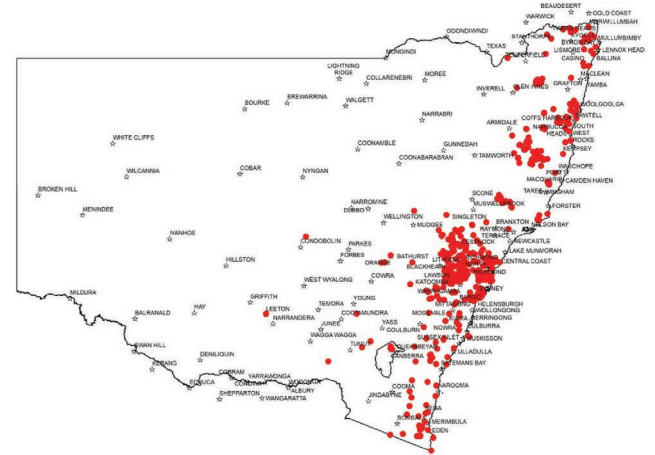
Fig. 3. Phytophthora cinnamomi presence records in NSW (to May 2020).
