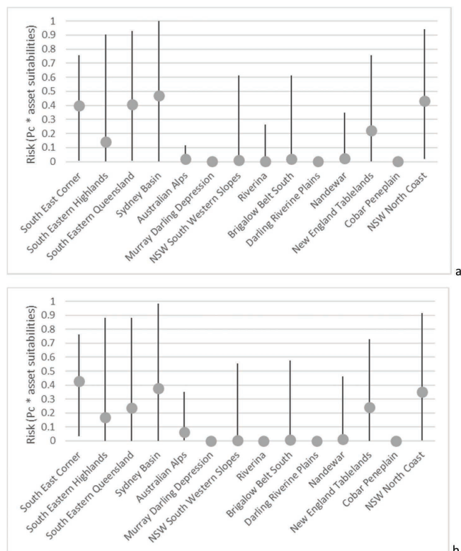
Fig. 14. Minimum to maximum risk for each IBRA region (line) and mean risk (grey dot), a) currently and b) in 2070 under representative concentration pathway 4.5.
