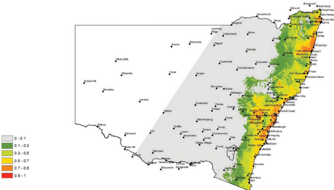
Fig. 11. Current risk to assets from the effects of Phytophthora cinnamomi . The map is the product of layers of habitat suitability for Phytophthora cinnamomi and assets (threatened species); 0 = no risk, 1 = highest risk.
