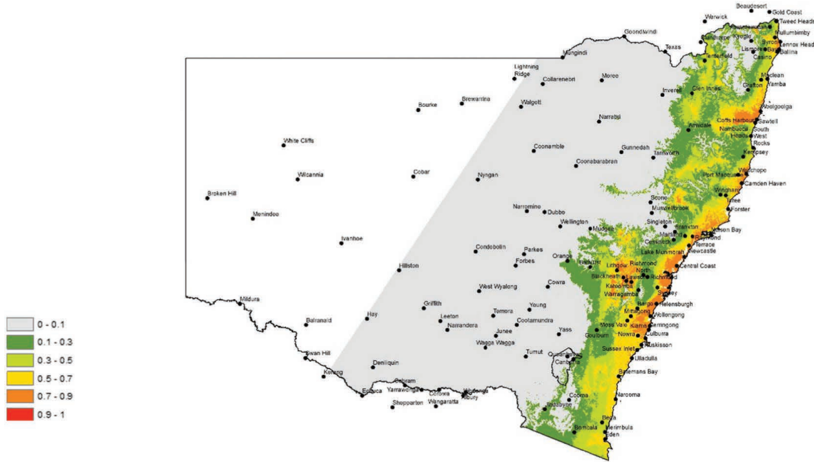
Fig. 12. Modelled risk to assets from the effects of Phytophthora cinnamomi in 2070 under representative concentration pathway 4.5. The map is the product of layers of habitat suitability for Phytophthora cinnamomi and assets (threatened species); 0 = no risk, 1 = highest risk.
