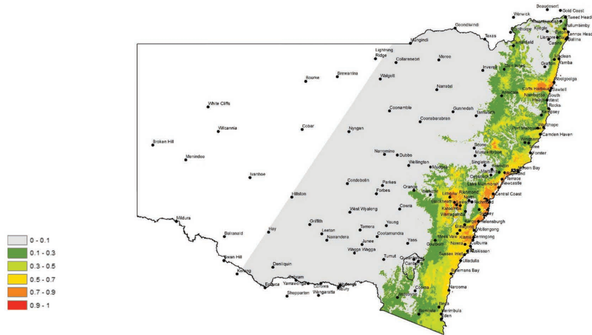
Fig. 13. Modelled risk to assets from the effects of Phytophthora cinnamomi in 2070 under representative concentration pathway 8.5. The map is the product of layers of habitat suitability for Phytophthora cinnamomi and assets (threatened species); 0 = no risk, 1 = highest risk.
