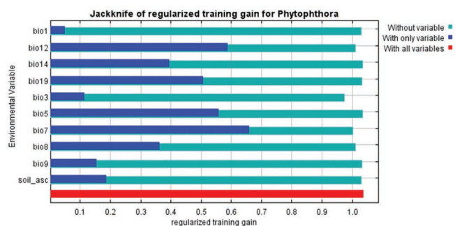
Fig. 6. Jackknife plots of variables included in the species distribution model created using MaxEnt. The red bar indicates the regularized training gain (i.e. how well the model predicts the presence data) from using all variables. The blue bars indicate the amount of training gain for each environmental variable alone while the green bars indicate the training gain when each environmental variable is omitted.
