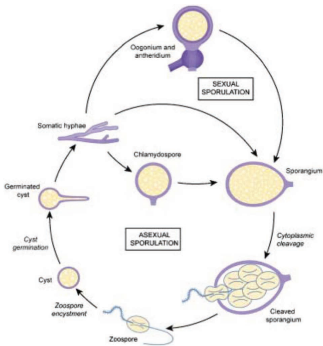
Fig. 1. Life cycle of Phytophthora cinnamomi . Reproduced with permission from Hardham (2005).
