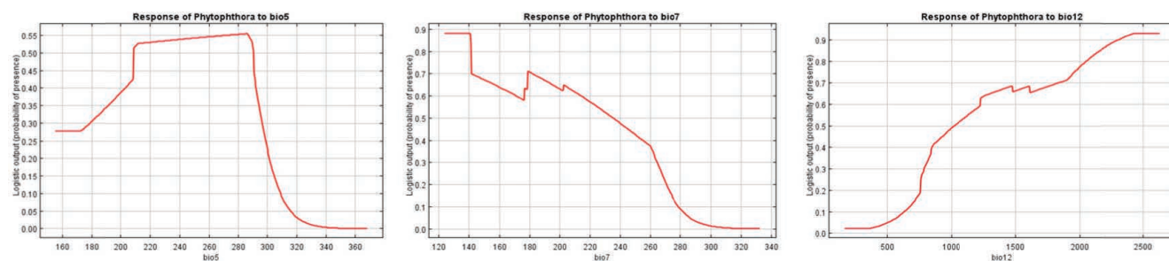
Fig. 5. Response curves of the most important variables in the model of suitability for Phytophthora cinnamomi (Bio5 = maximum temperature of warmest month, Bio7 = temperature annual range, Bio12 = annual precipitation). Note that for Bio5 and Bio7, temperature values on the x axis are multiplied by 10.
