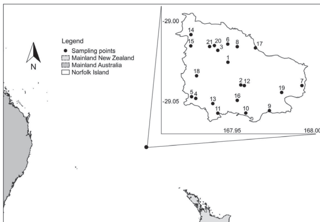
Fig. 1. Location of Norfolk Island in the South Pacific and locations of actual sampling sites on the island.
