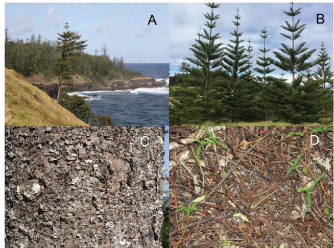
Fig. 2. (A) Coastline of Norfolk Island. (B) Young Norfolk Island pines. (C) Bark surface of Norfolk Island pine. (D) Forest floor leaf litter.
