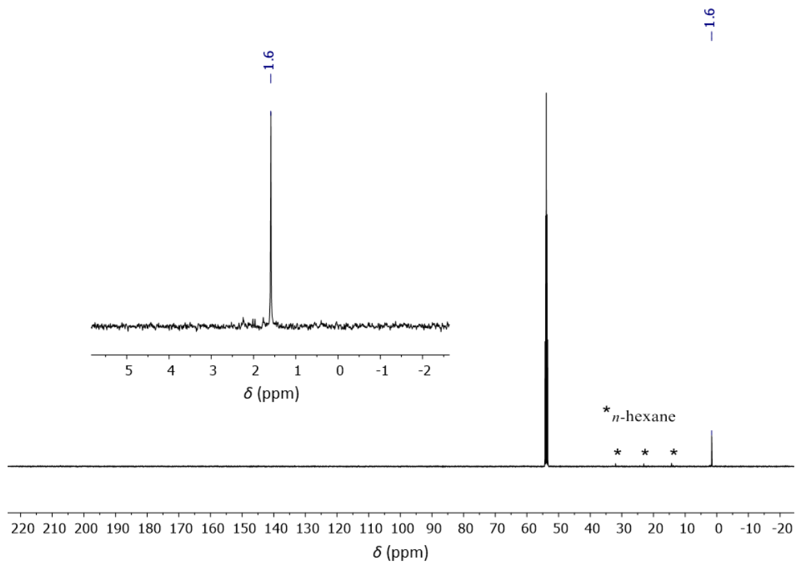
Figure S8. ^{13}\text{C}\{^1\text{H}\} NMR spectrum of [2] ( \text{CD}_2\text{Cl}_2 , 125.8 MHz); * n -hexane.
