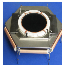
Figure 5. Left: delay-line anode structure. Right: complete delay-line detector with microchannel plates (black area) and holder. [14]
