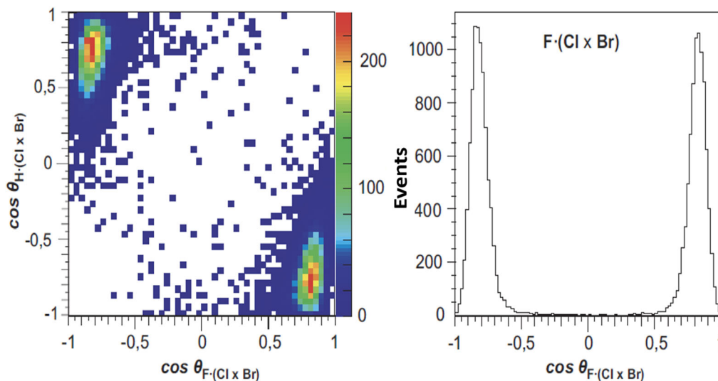
Figure 34. Measured handedness distribution as function of the chirality parameter \cos \Theta_{F(\text{Cl} \times \text{Br})} = p_F \cdot (p_{\text{Cl}} \times p_{\text{Br}}) / (|p_F| \cdot |p_{\text{Cl}} \times p_{\text{Br}}|) . [57,58]
