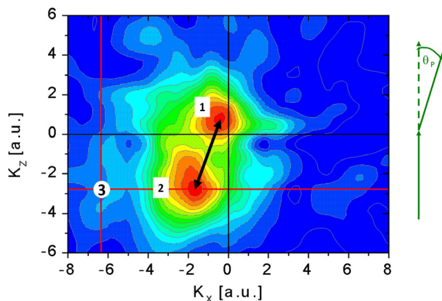
Figure 9. \text{He}^{2+} recoil-ion momentum distribution in the nuclear scattering plane for the transfer ionization process 1 MeV Proton projectiles on \text{He} . [19] Right: The direction of the \text{H}^{\circ} deflection. The \text{H}^{\circ} scattering angle \theta_p is 0.55 mrad. The kinetic energy difference of the recoil ions between the two peaks 1 and 2 is about 65 meV. The momentum resolution is about 0.1 a.u. and thus the recoil energy resolution about 1 meV. [19]
