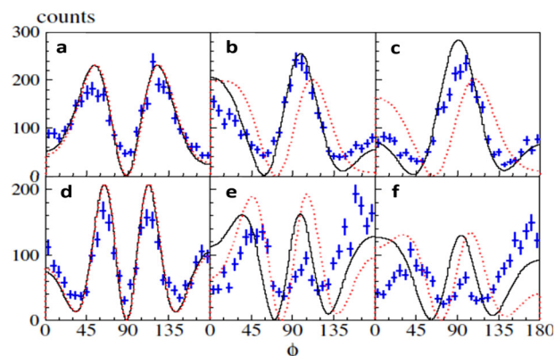
Figure 13. Relative cross-sections as function of the angle \varphi in comparison with model calculations (red dashed lines) and full theory (solid lines). [26] The left column represents collisions where \theta is from 85^\circ to 90^\circ , the middle column where \theta is from 55^\circ to 60^\circ and the right column where \theta is from 45^\circ to 50^\circ . The rows show data for different transverse momenta and slightly different KER values.
