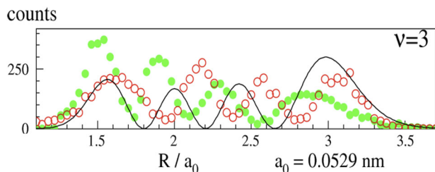
Figure 18. Spatial density of the vibrational state \nu = 3 (see text). [30]
