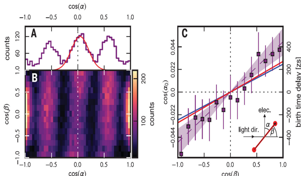
Figure 35. Left: interference pattern of photoelectrons emitted from H_2 horizontal axis emission angle of the electron with respect to the molecular axis, vertical axis: angle between the molecular axis and the light propagation direction. If the photoelectron wave would start at the same time from both centers of the molecule the central maximum would be at \cos(\alpha) = 0 . From the observed shift the time delay between the emission from one to the other center can be deduced. Right: shift of the central interference fringe (left axis) and the corresponding time delay (right axis) as function of the molecular orientation to the light propagation axis. The blue line shows the expectation in case of a delay given by the speed of light, the red and dashed lines show the best linear fits through the data. Adapted with permission. [61] Copyright 2020, AAAS.
