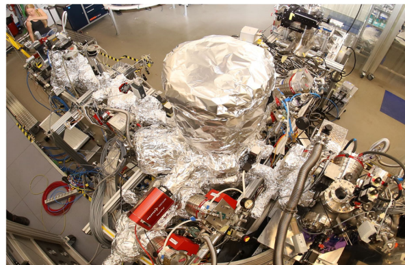
Figure 6. C-REMI system of the Frankfurt group mounted at the European XFEL. [15]
